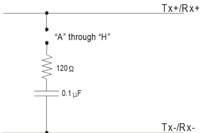
Figure 3-1: Simplified Termination Schematic
