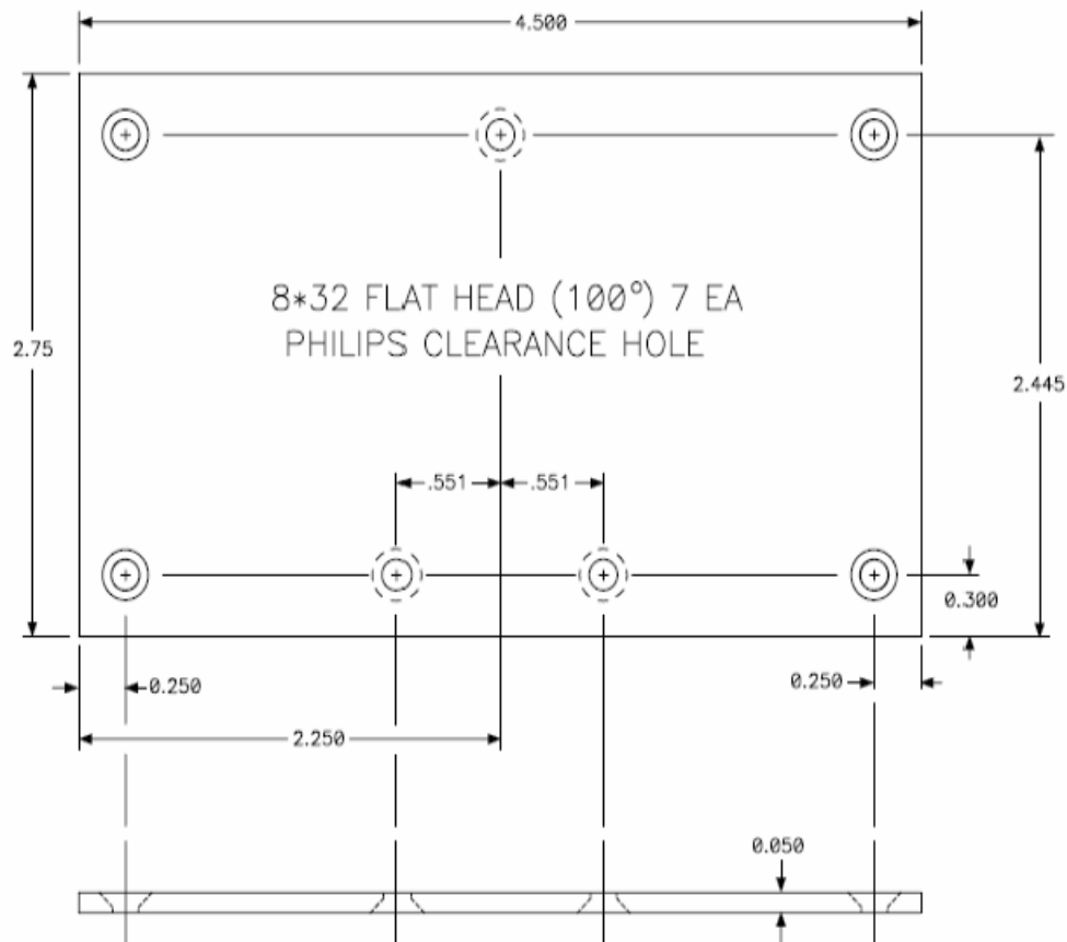
Figure 2-4: DPK-MOUNT
