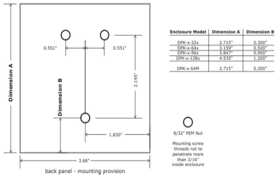
Figure 2-2: DAQ-PACK Mounting Provisions
