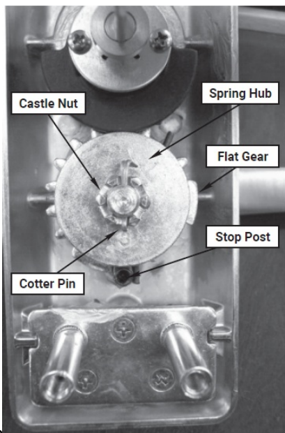
Left-Hand Reverse
