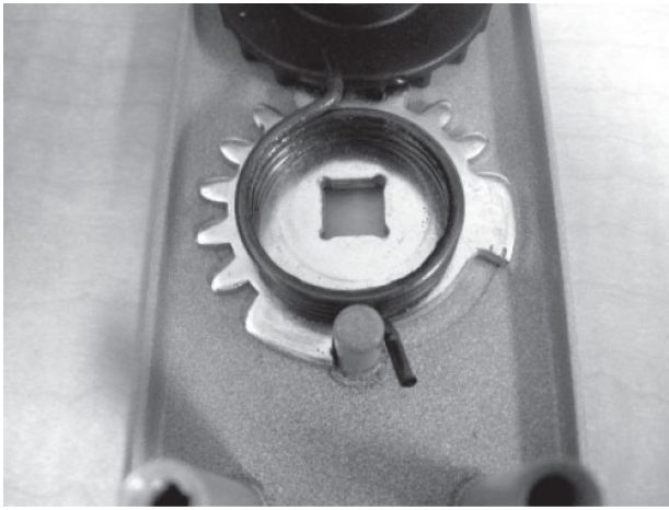
Right Hand Reverse Gear & Spring Orientation
