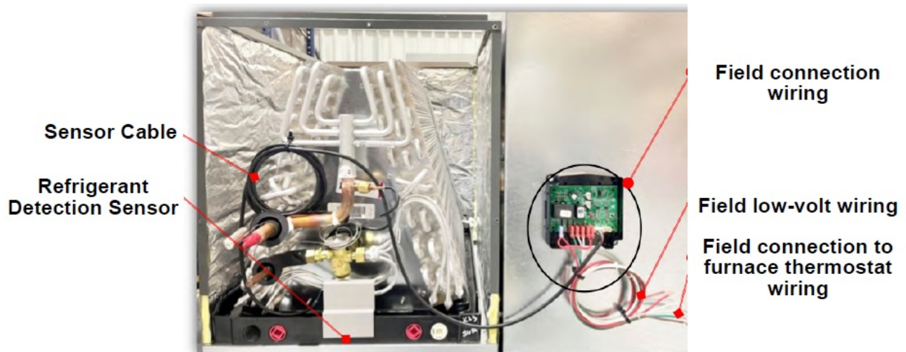
Figure A1 – Mitigation Control Boards (cover removed to show internal components)
