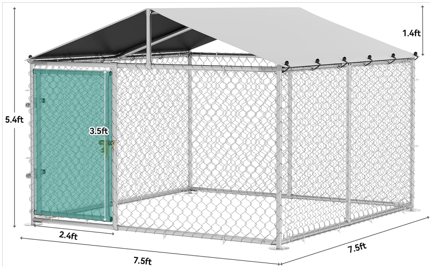
Image 4.1: Dimensional overview of the YITAHOME Outdoor Dog Kennel.
