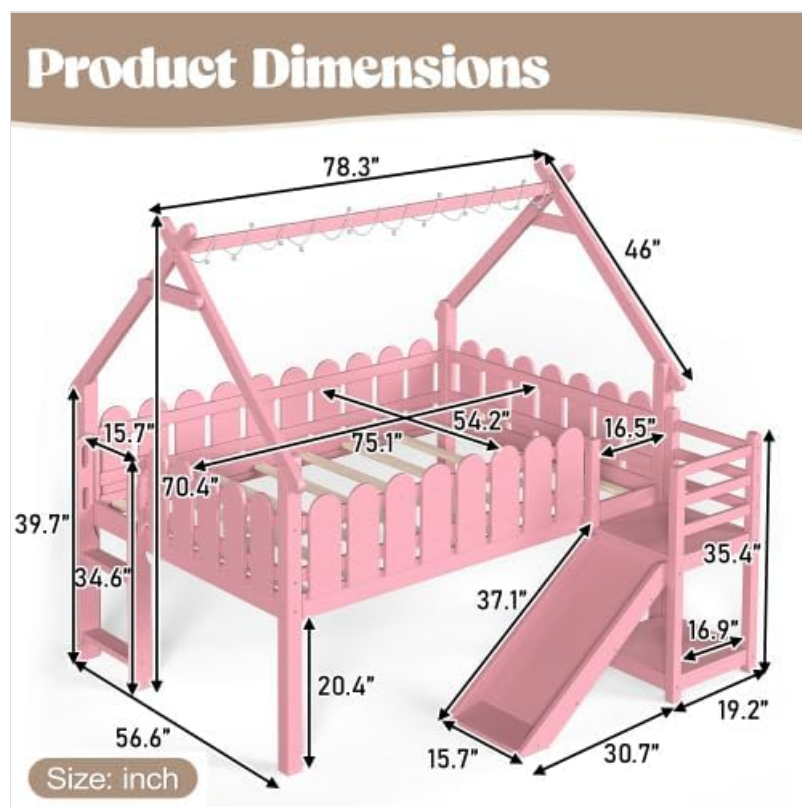
Figure 1: Product Dimensions. This diagram illustrates the overall dimensions of the Bellemave Low Loft Bed, including length, width, and height, as well as specific measurements for the slide, ladder, and bed frame components. All measurements are in inches.
