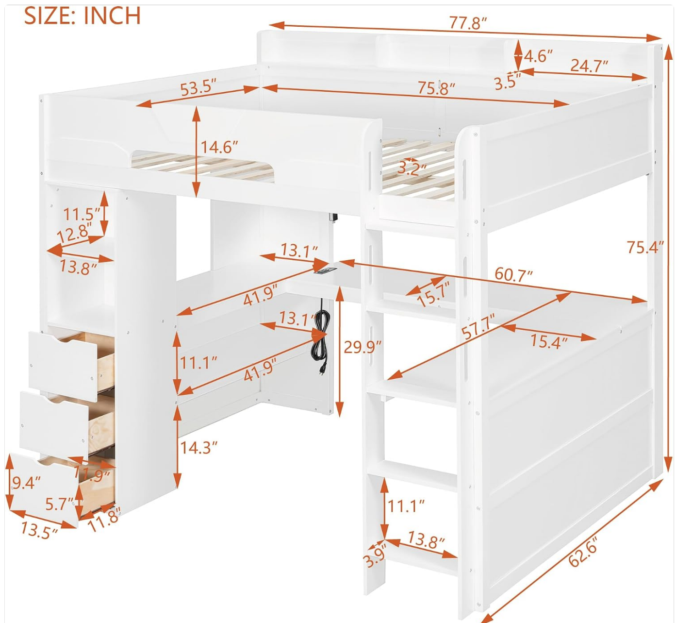
Image: Detailed dimension diagram of the loft bed, illustrating overall size and component measurements for planning assembly space.
