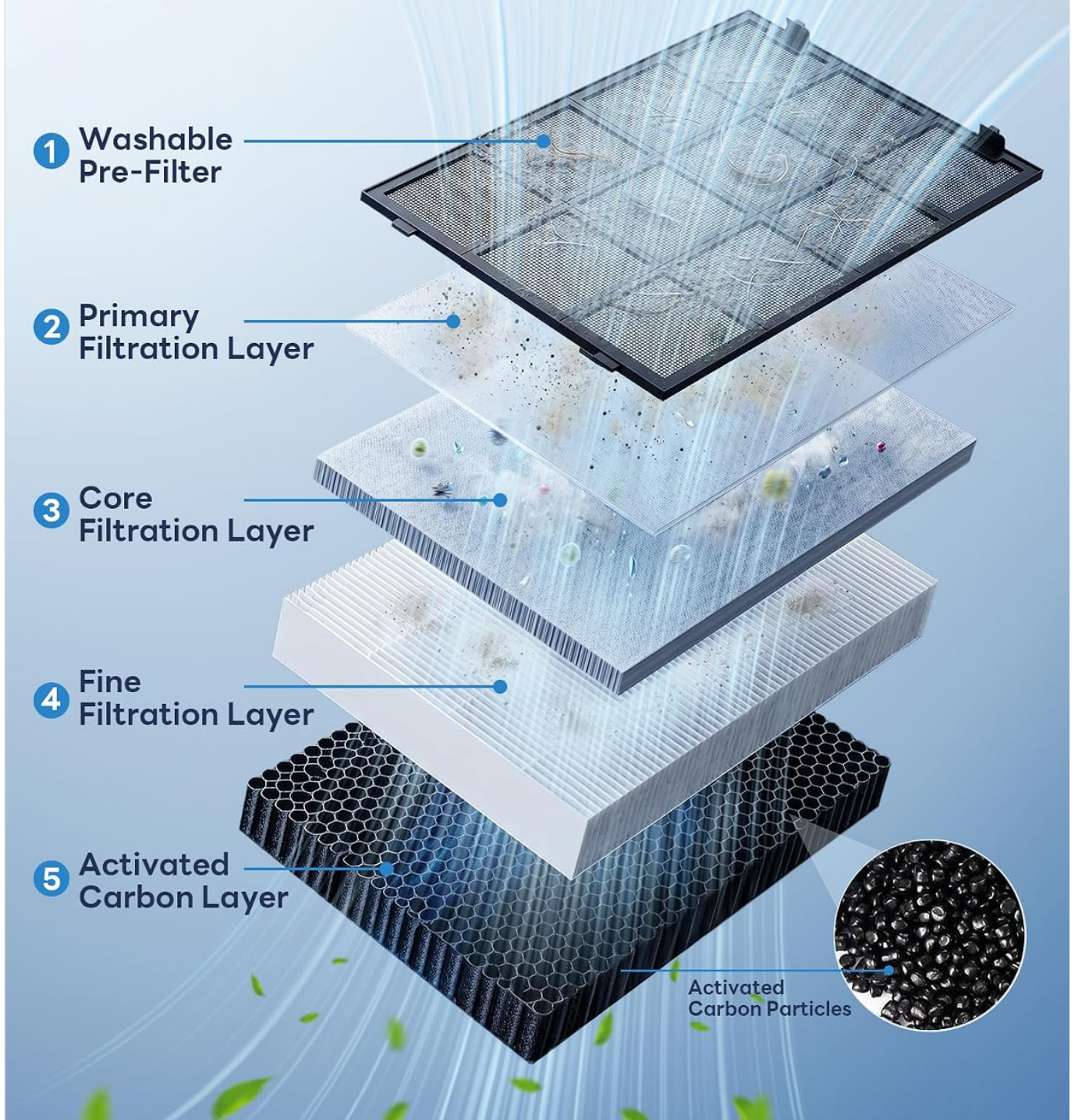
Figure 3.1: Detailed view of the 5-Stage Filtration System
