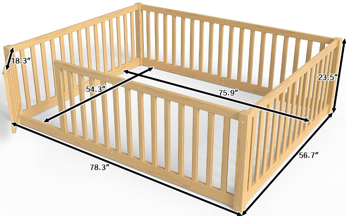
Figure 2: This diagram illustrates the overall dimensions of the assembled floor bed, including length, width, and height of the frame and door opening.
