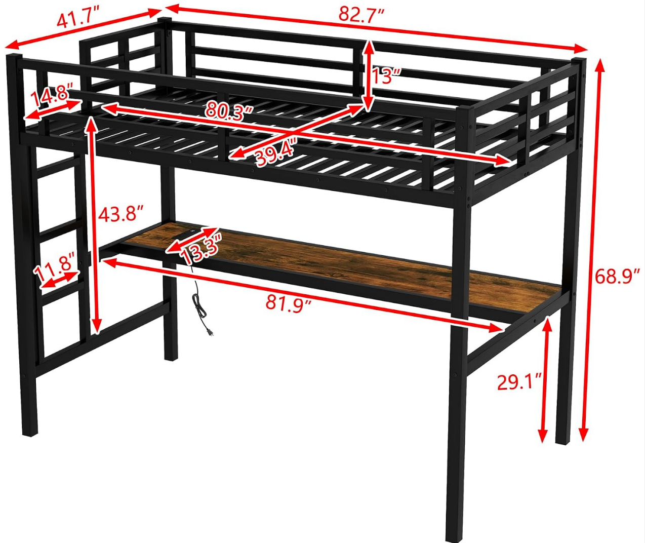
Image 1: Dimensional diagram of the Bellemave Metal Twin XL Loft Bed, illustrating overall length, width, height, and specific measurements for the bed frame, desk, and ladder. This helps in identifying parts and understanding the bed's structure during assembly.
