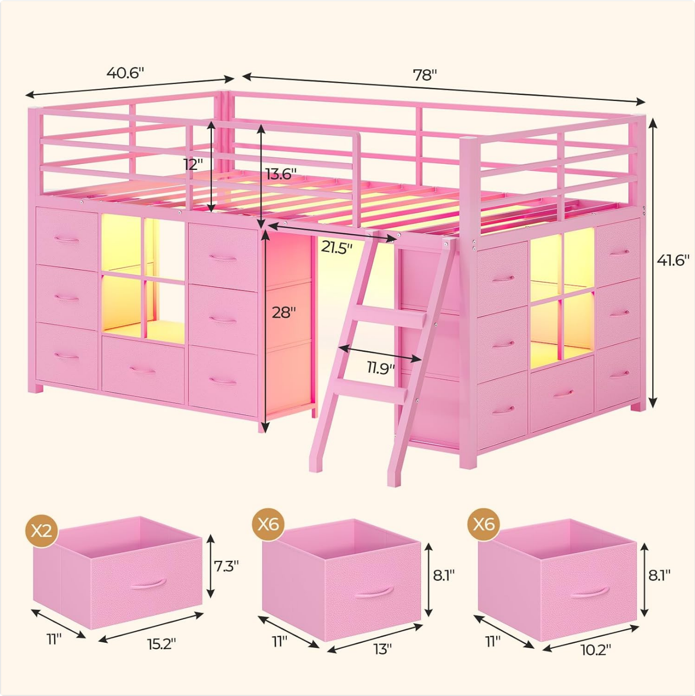
Image: Detailed dimensions of the loft bed, including overall length, width, height, and individual drawer sizes.
