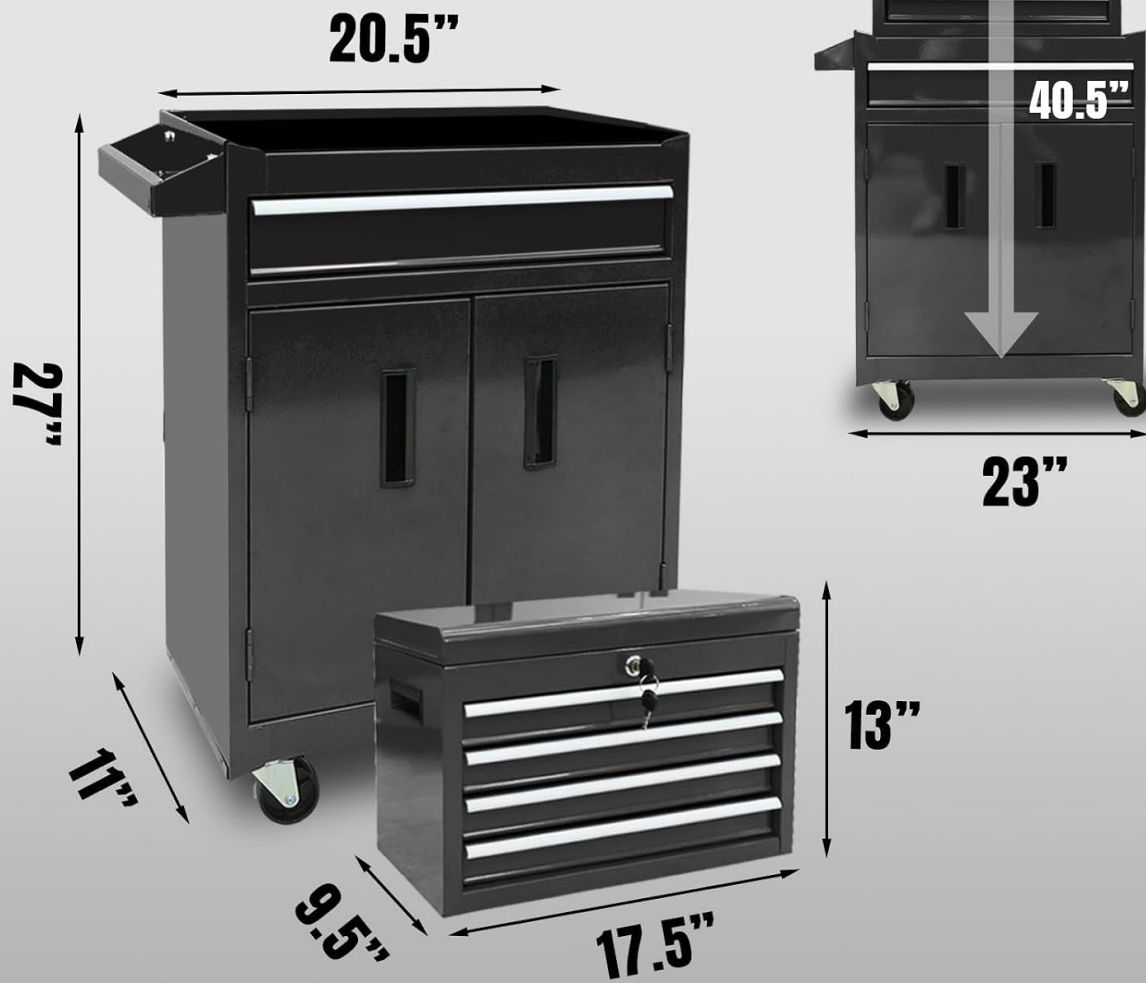
Figure 1: Product Dimensions and Detachable Components. This image illustrates the overall dimensions of the assembled unit, as well as the individual dimensions of the detachable top tool chest and the rolling bottom cabinet.
