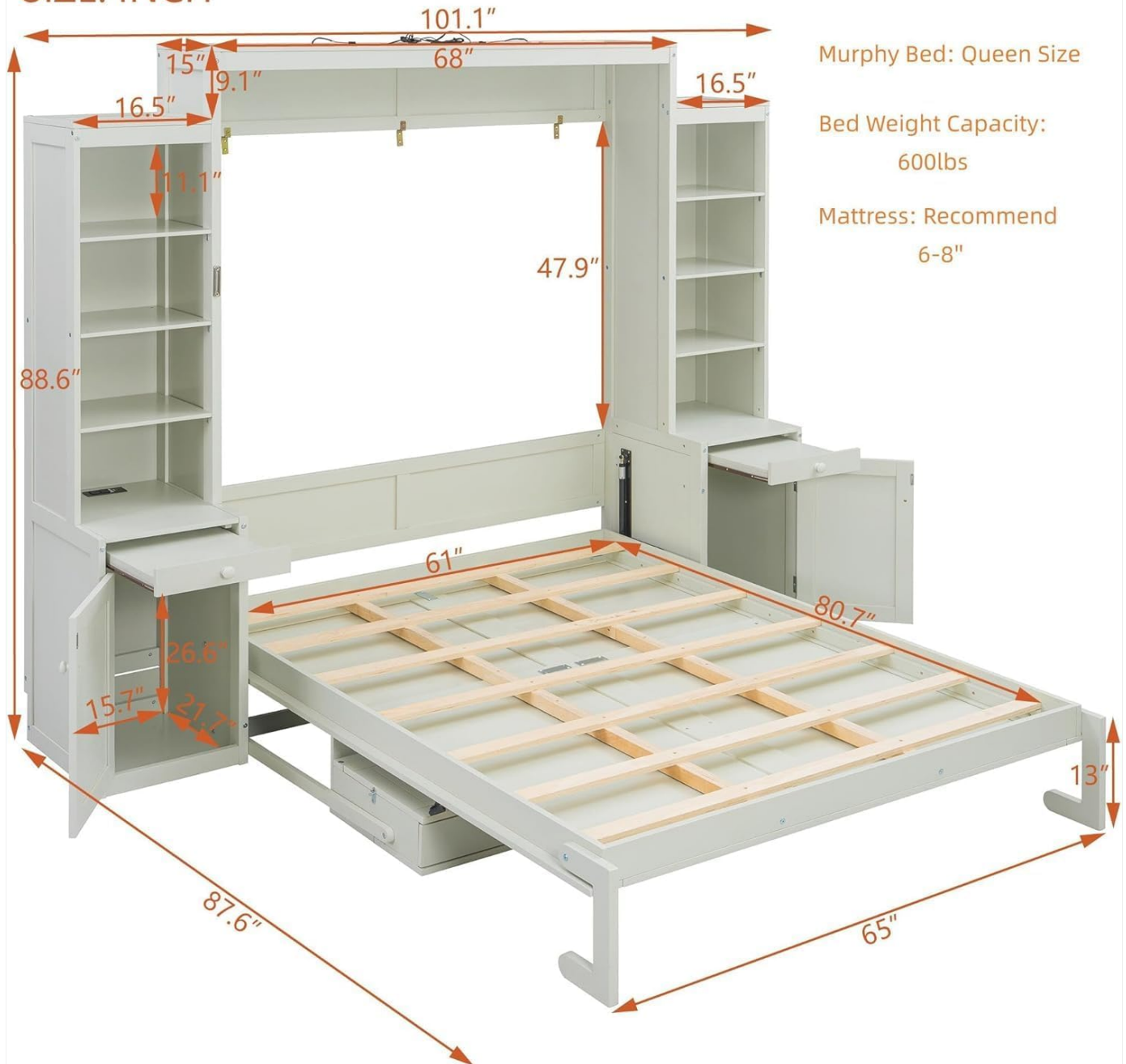
Figure 1: Product Dimensions Overview. Refer to this diagram for overall measurements and component sizes.
