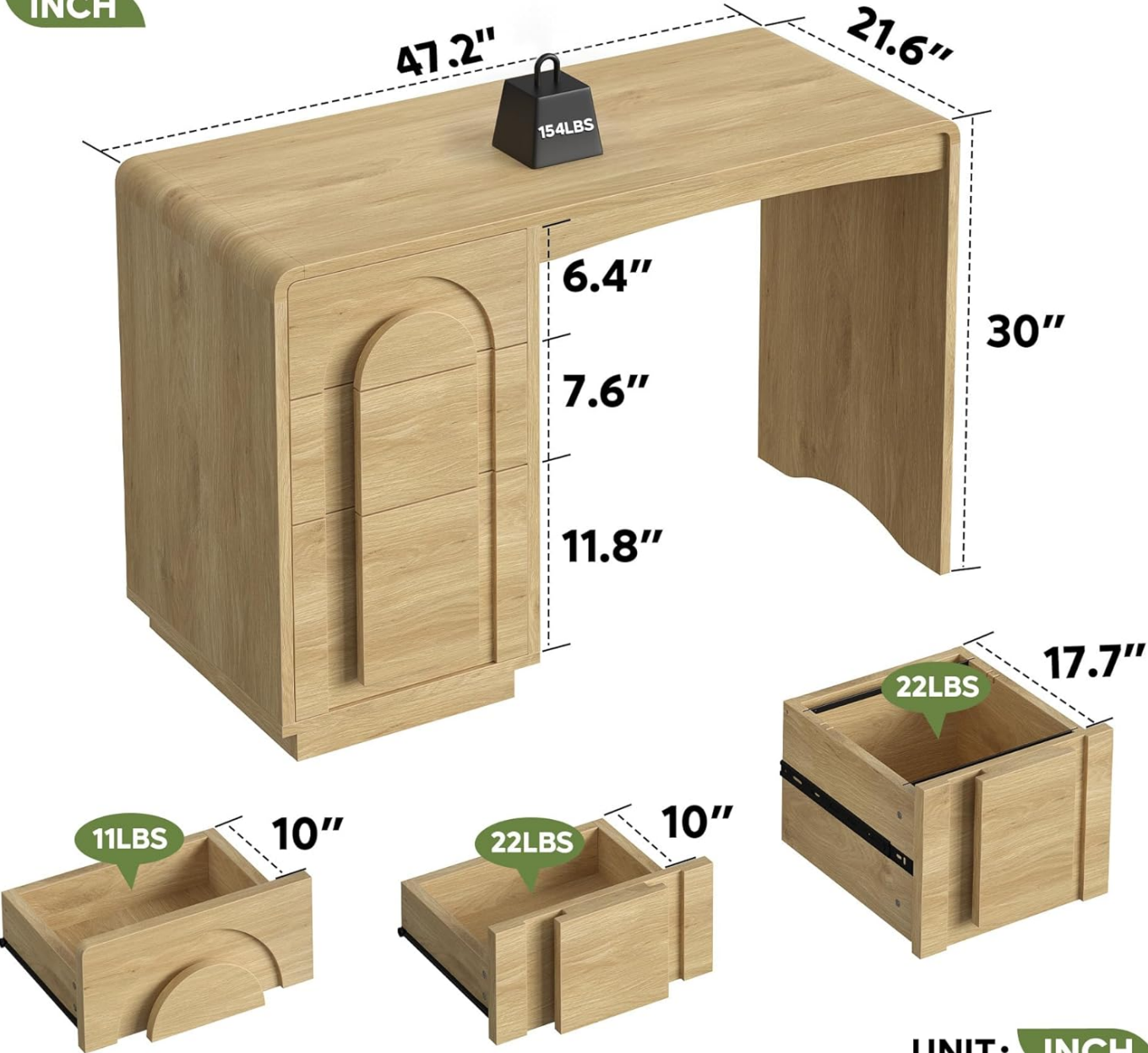
Image: Diagram illustrating the product dimensions and individual drawer weight capacities.
