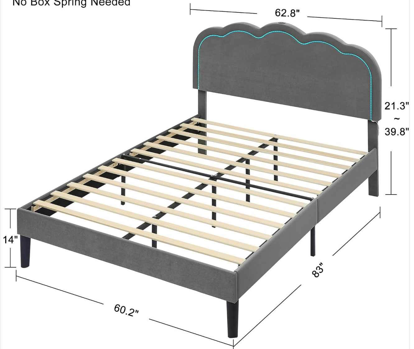
Image: Dimensional diagram of the VECELO Queen Size Bed Frame, illustrating length, width, height, and under-bed clearance.
