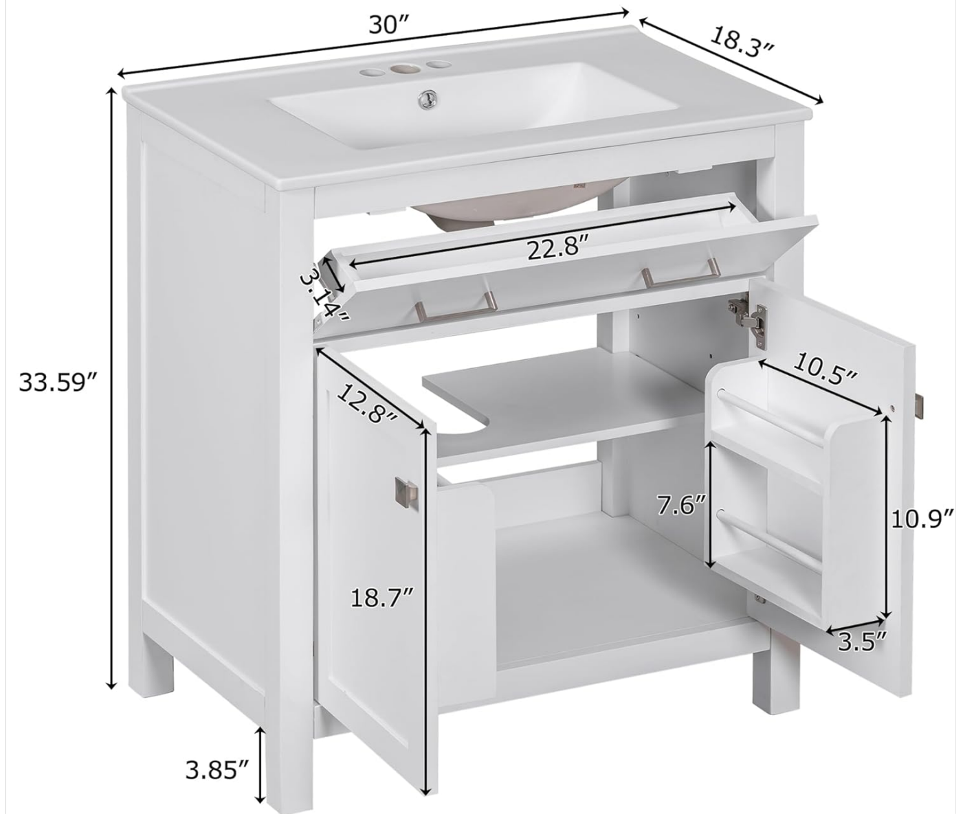
Detailed dimensions of the vanity cabinet and sink in inches.
