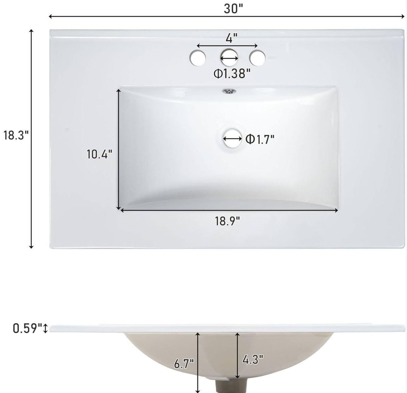
Detailed dimensions of the ceramic sink, including faucet hole spacing.
