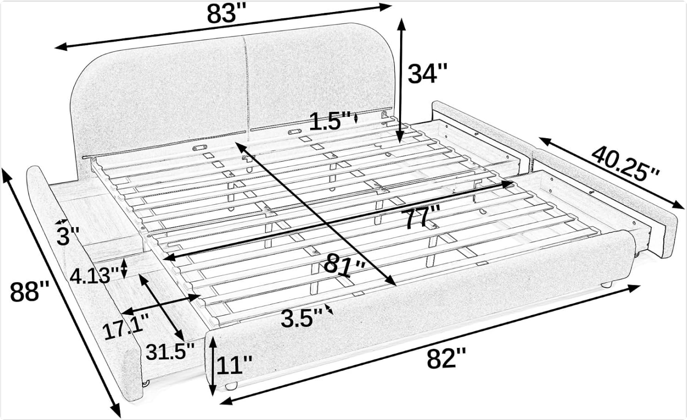
Image: Technical diagram displaying the precise dimensions of the roomfitters King Size Bed Frame.
