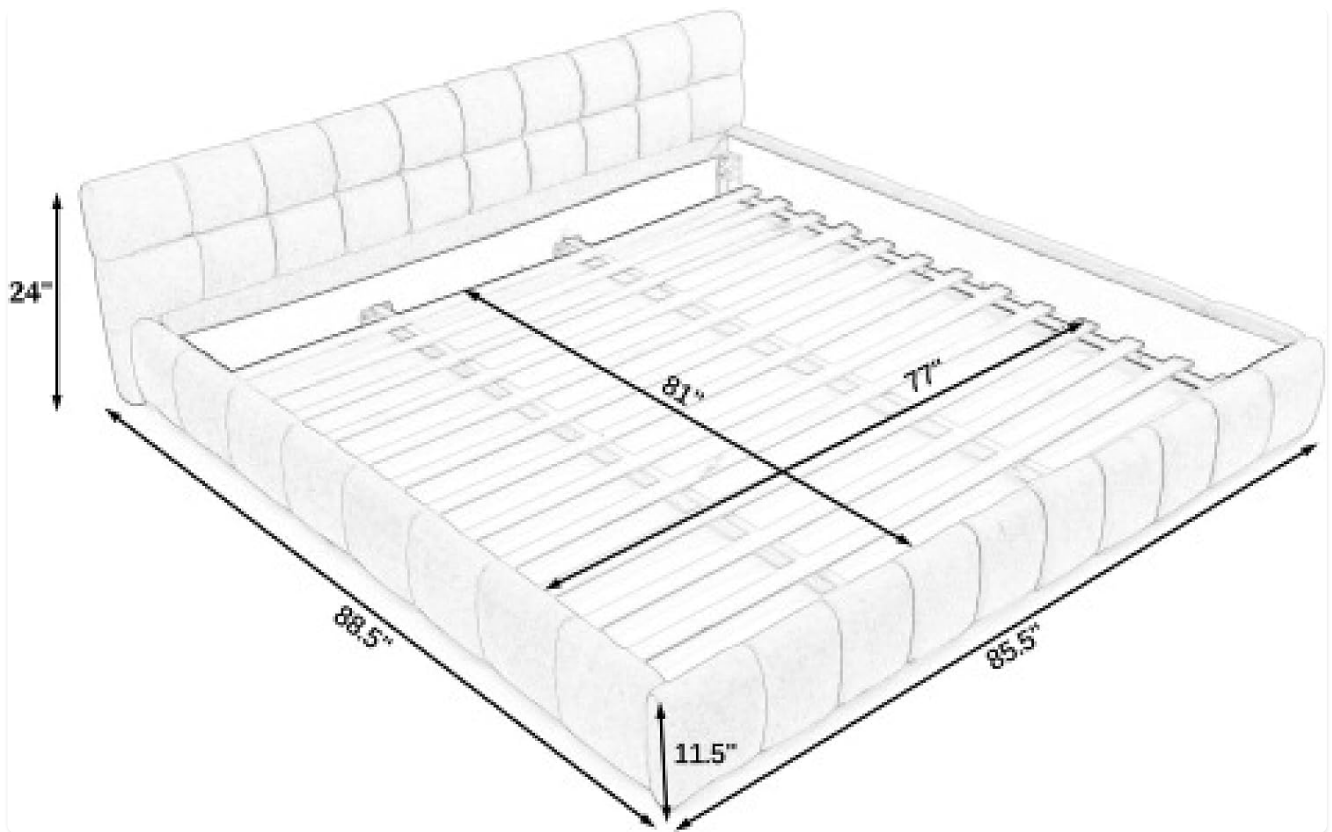
Image 3: Dimensional diagram of the roomfitters King Size Upholstered Bed Frame.
