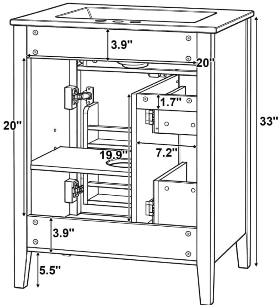
Image: Back view diagram with detailed measurements, showing the open back for plumbing connections.
