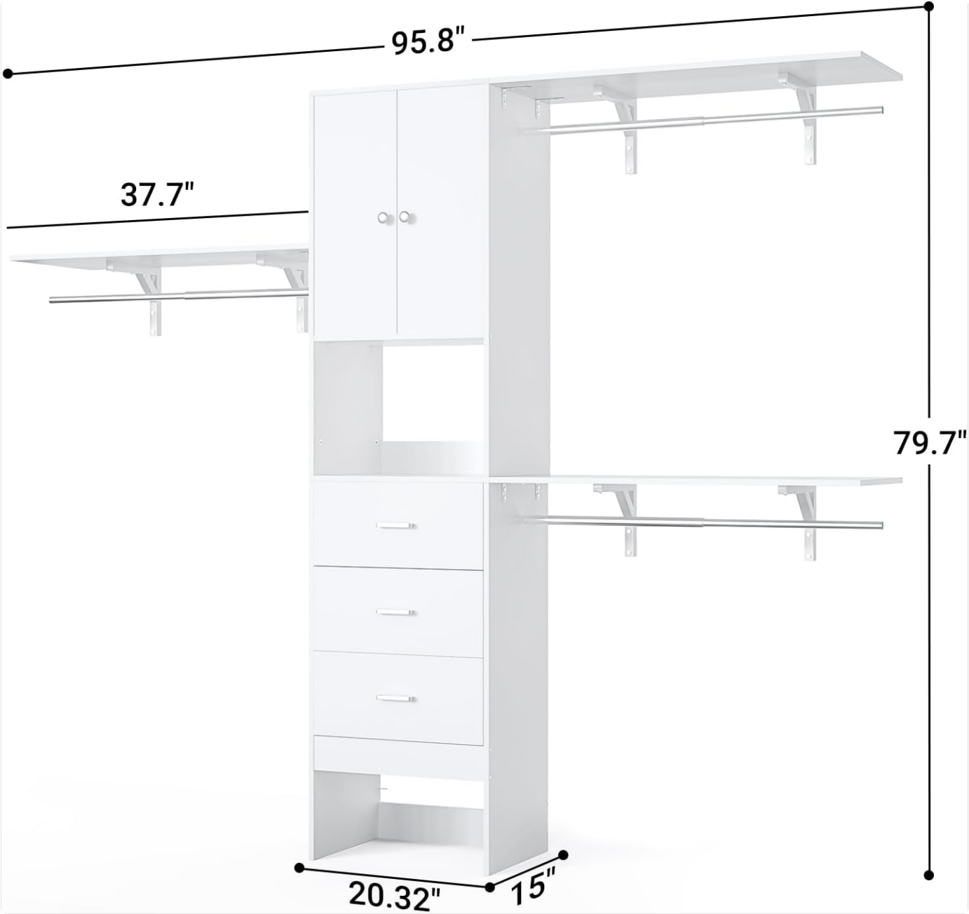
Figure 8.1: Product Dimensions. This diagram provides key measurements for the closet system, including overall length, height, and individual tower dimensions.
