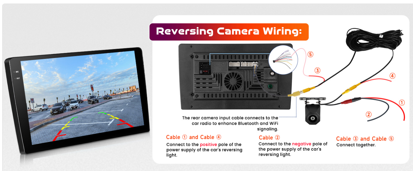
Figure 4: Reversing camera wiring instructions.
