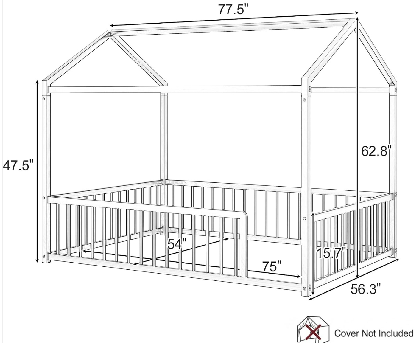
Image: Technical drawing showing the full dimensions of the bed frame in inches.
