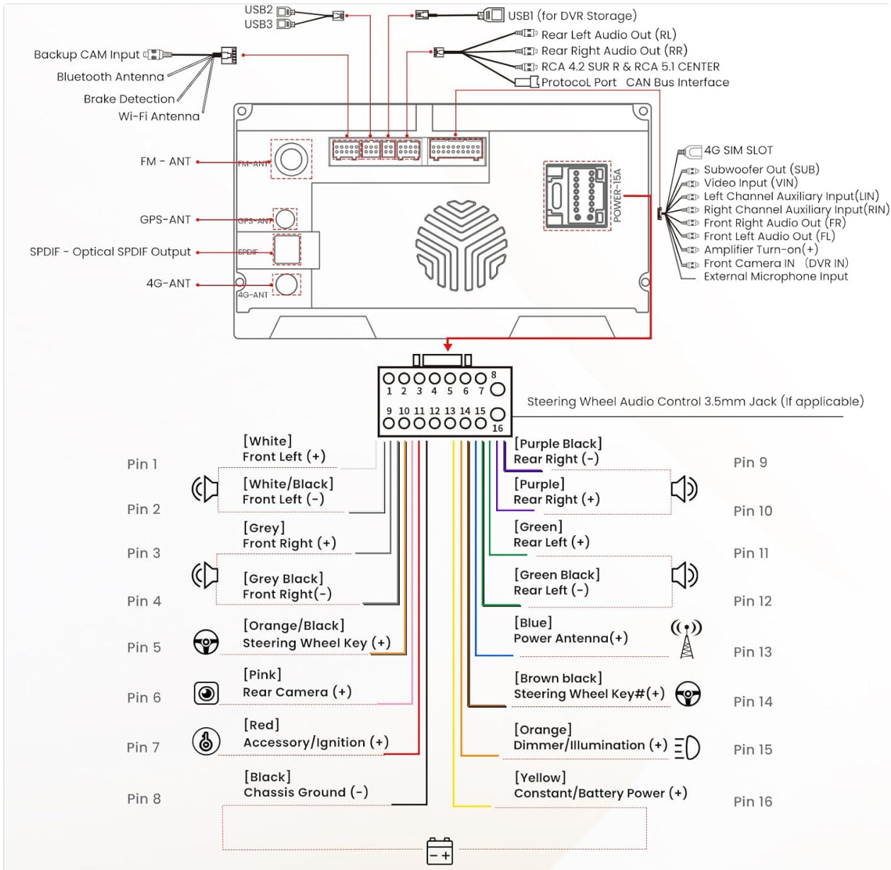
Figure 4.1: ATOTO S8L Wiring Diagram
