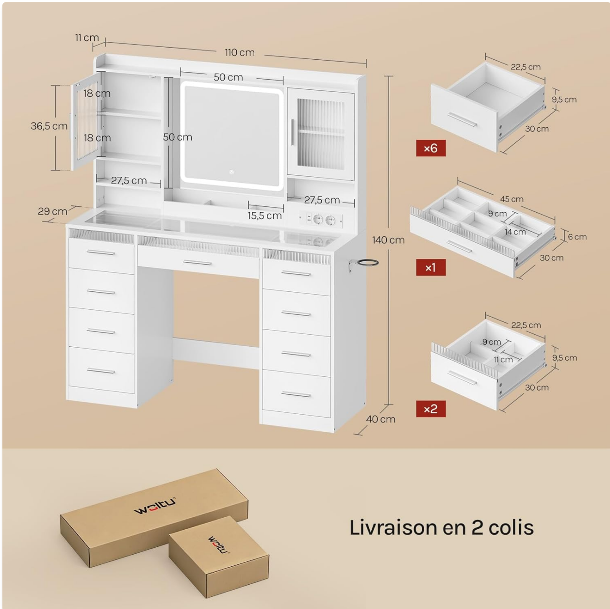
Image 3.1: An exploded view diagram illustrating the overall dimensions of the dressing table (110 cm width, 40 cm depth, 140 cm height) and the individual sizes of the six standard drawers, one large partitioned drawer, and two smaller partitioned drawers. The image also shows two boxes indicating the product ships in two packages.
