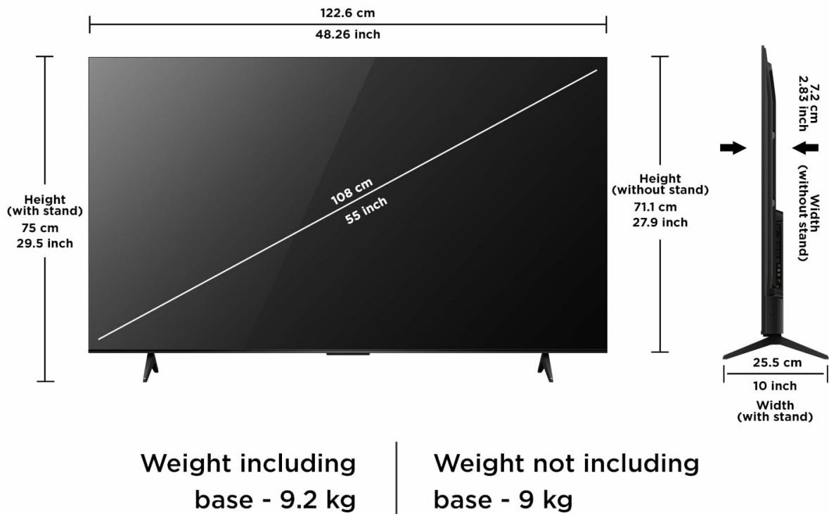
Image: Diagram illustrating the dimensions and weight of the TCL 55T6D television, both with and without its stand, for installation planning.
