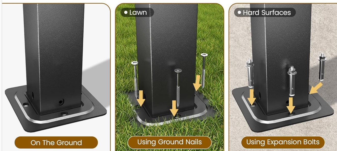
Image 4.2: Ground fixing options for various surfaces.
