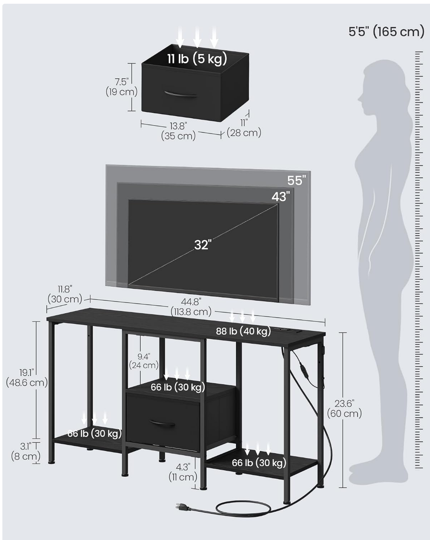
Image: A comprehensive diagram illustrating the dimensions and maximum static load capacities for various sections of the TV stand.
