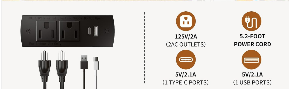
Figure 6: Built-in multifunctional socket with 2 AC outlets (125V/2A), 1 USB-A port (5V/2.1A), and 1 USB-C port (5V/2.1A), featuring a 5.2-foot power cord.
