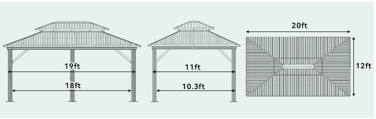
Image: Gazebo dimensions for planning your installation space.
