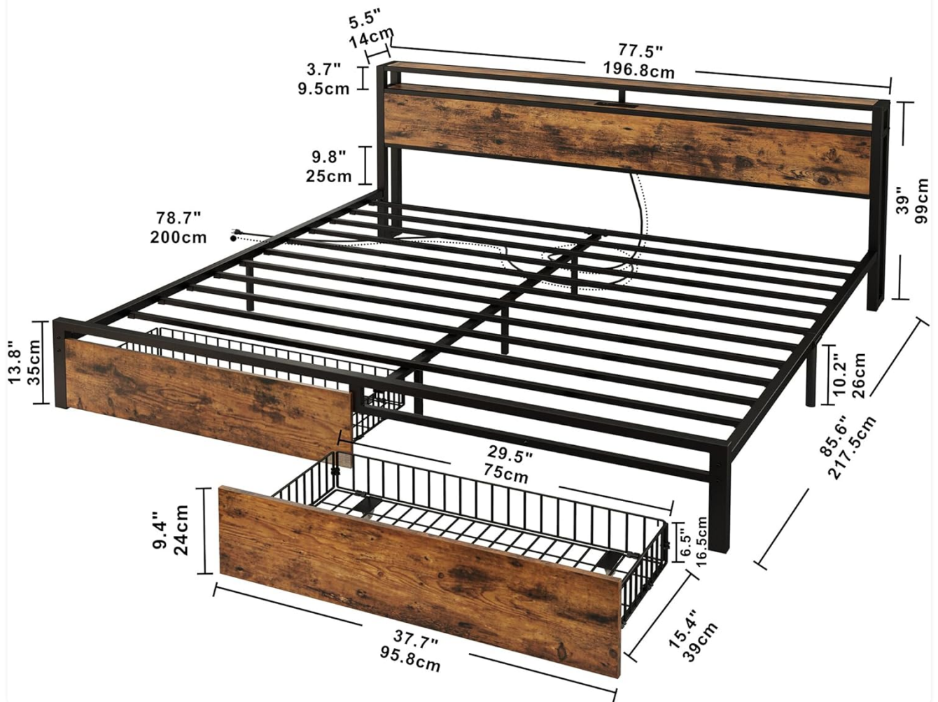
Image: A detailed diagram illustrating the dimensions and components of the King Size Bed Frame.
