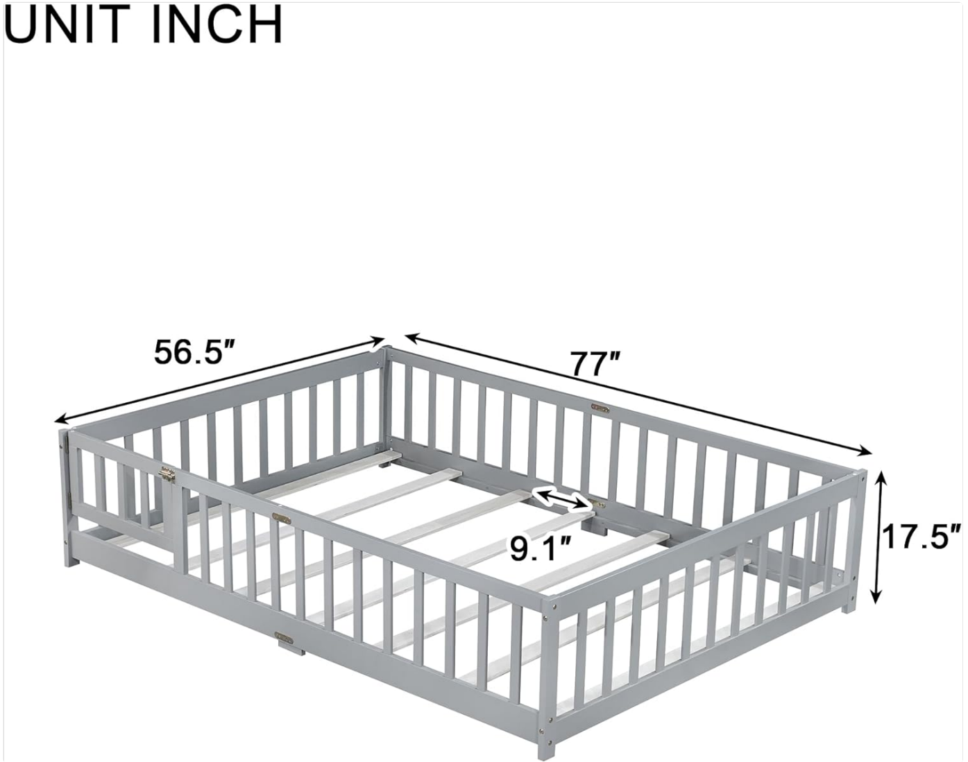
Image 4.1: Dimensional diagram of the Flieks Full Size Floor Bed, showing overall length (77"), width (56.5"), and height (17.5").
