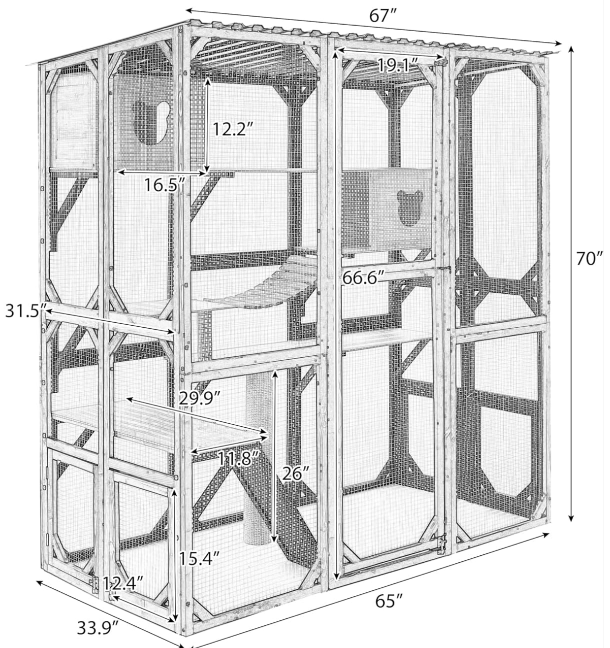
Image 4.1: Dimensional overview of the cat enclosure, useful for understanding component placement during assembly.
