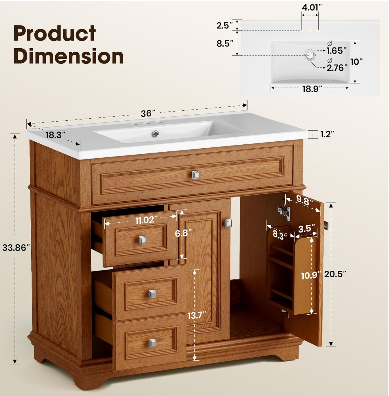
Image: Detailed product dimensions for the 36-inch vanity, including sink and cabinet measurements.
