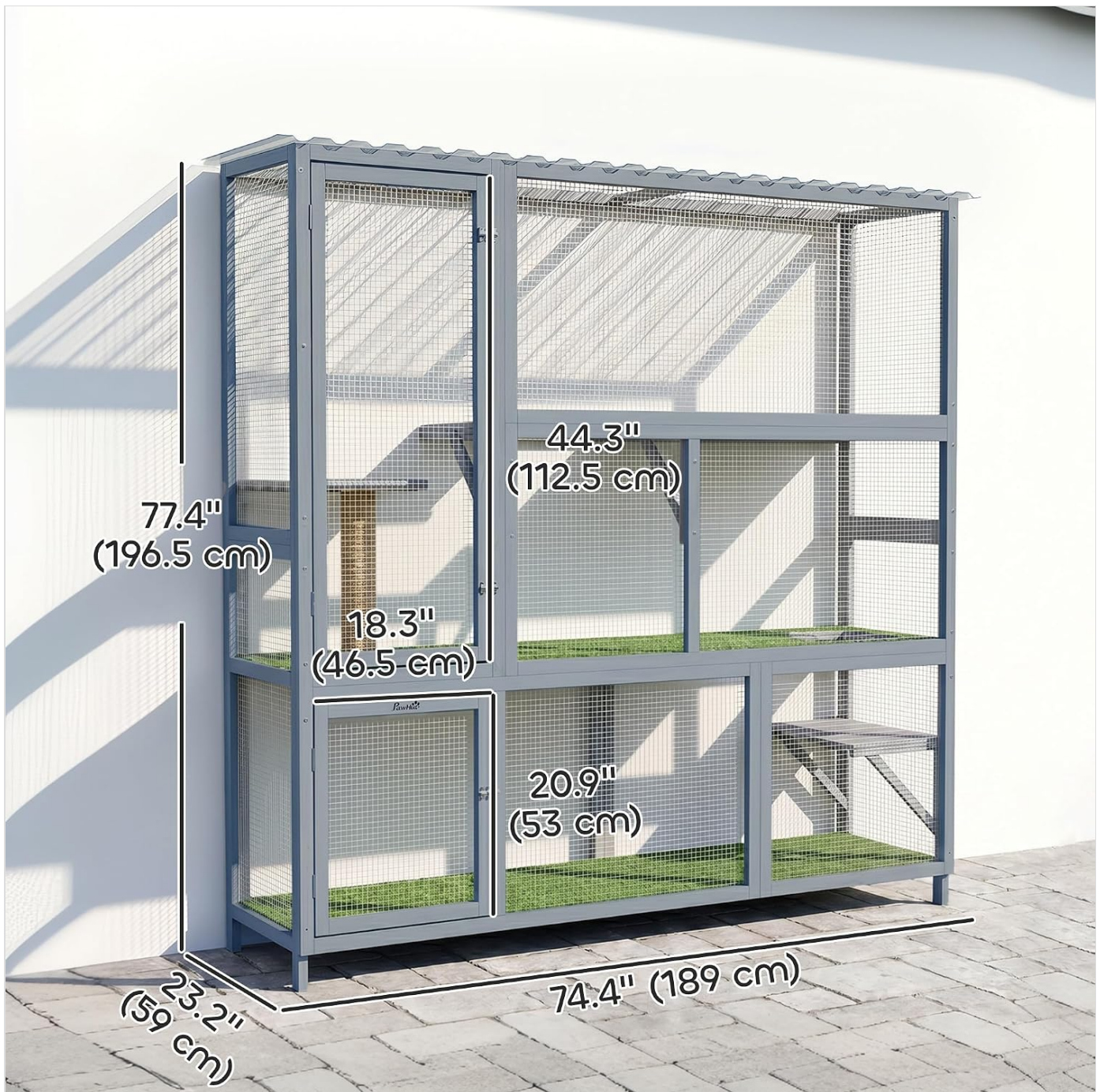
Figure 7: Detailed dimensions of the catio for planning placement.
