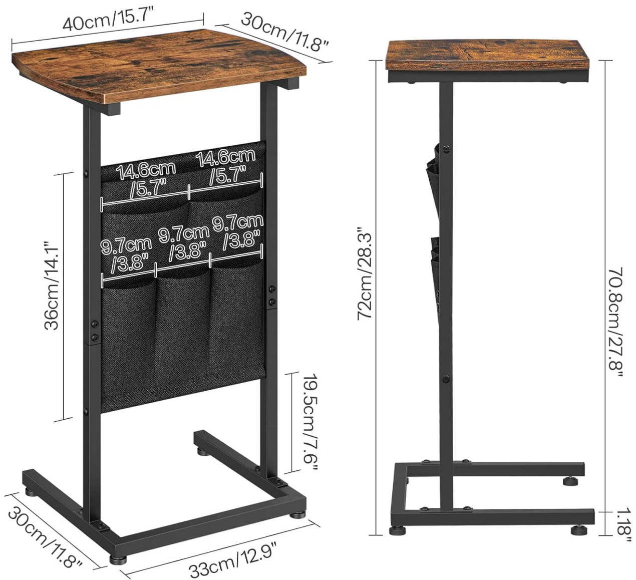
Image 8.2: Detailed dimensions of the HOOBRO C Shaped End Table.
