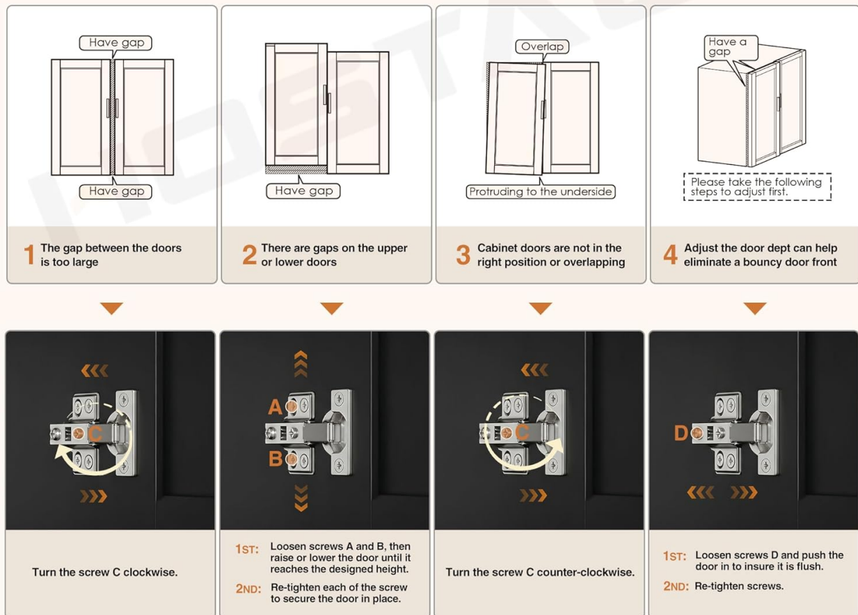
Figure 2: Step-by-Step Hinge Adjustment. This diagram illustrates how to fix common cabinet door alignment issues such as gaps, overlaps, and protruding doors by adjusting screws A, B, C, and D on the hinges.
