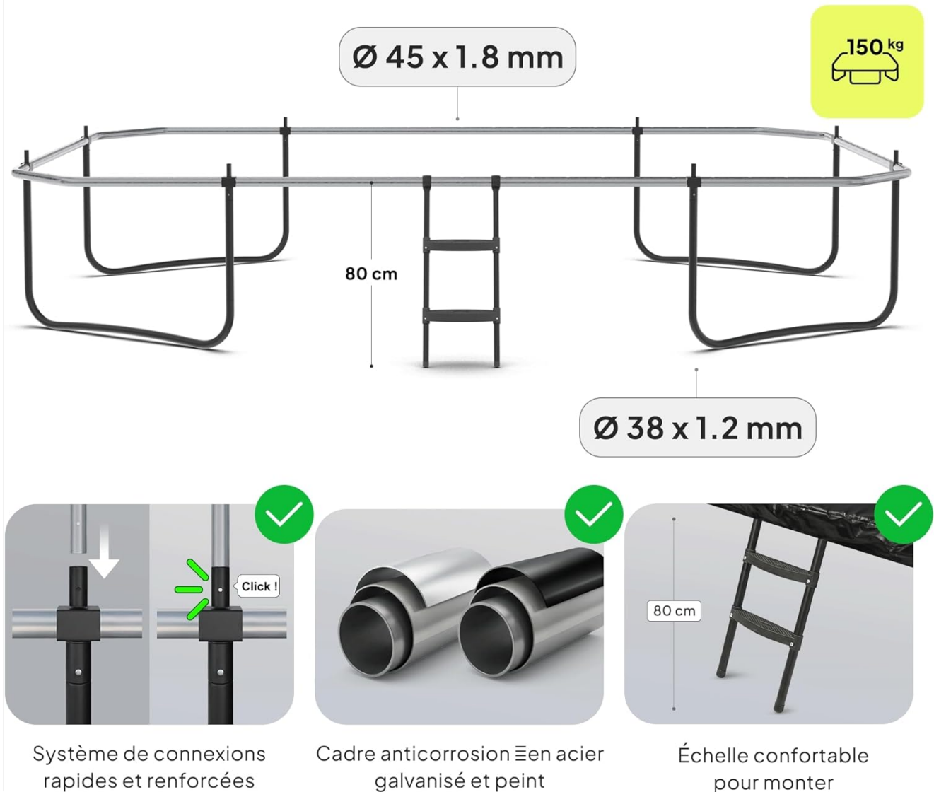
Image: A technical illustration detailing the trampoline's corrosion-resistant frame construction, featuring quick and reinforced connection points (indicated by "Click!"), galvanized and painted steel tubes ( \varnothing 45 \times 1.8 \text{ mm} and \varnothing 38 \times 1.2 \text{ mm} ), and the 80 cm high access ladder.
