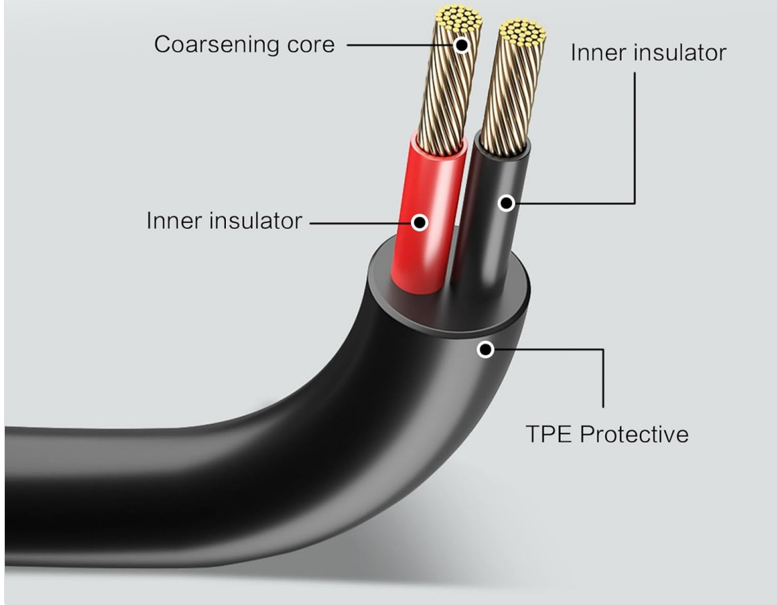
Image: Internal structure of the premium cable, designed for durability.
