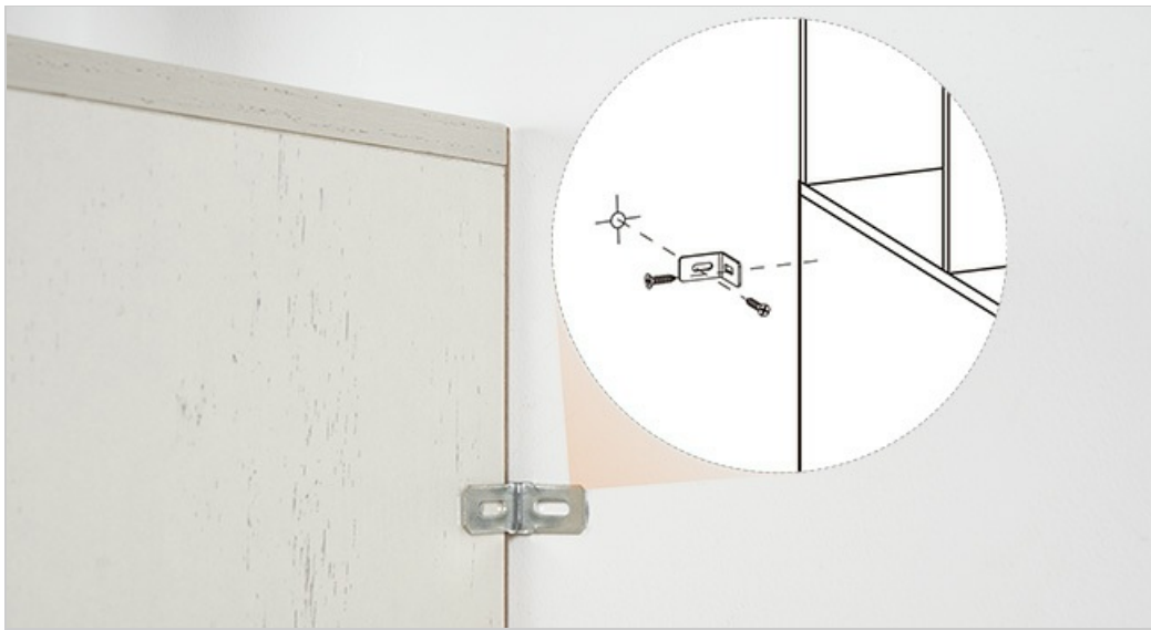
Image: Detailed view of the anti-tip kit and its installation process.
