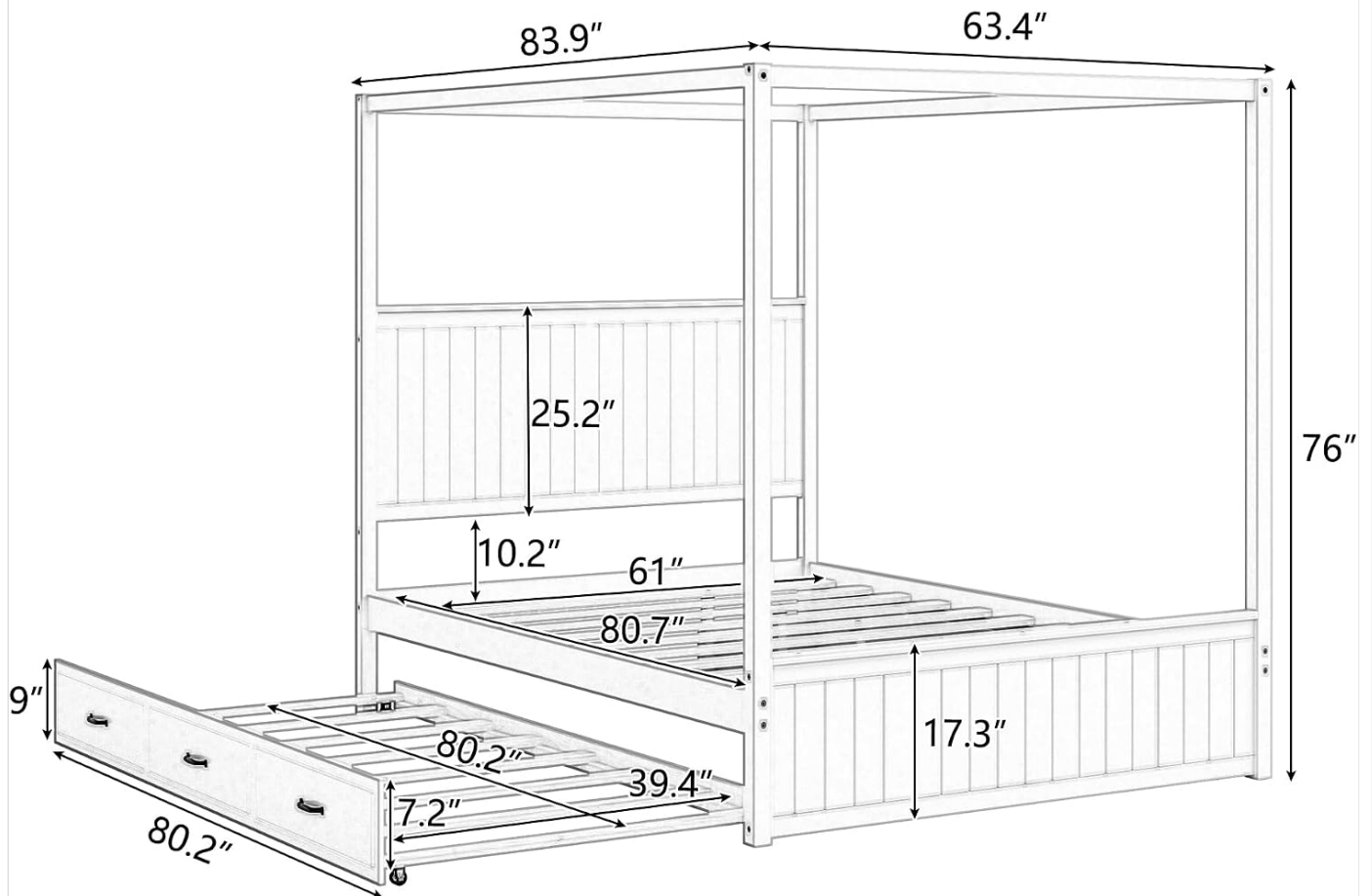
Figure 5: Detailed dimensions diagram for the Merax Queen Size Canopy Platform Bed and its components.
