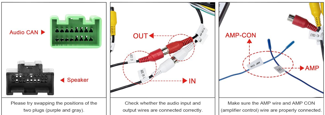
Image 3.3: General plug connection instructions.
