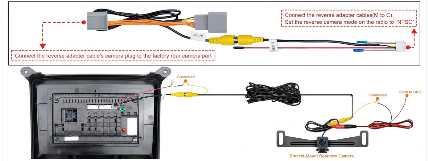
Image 3.2: Backup camera wiring diagram.
