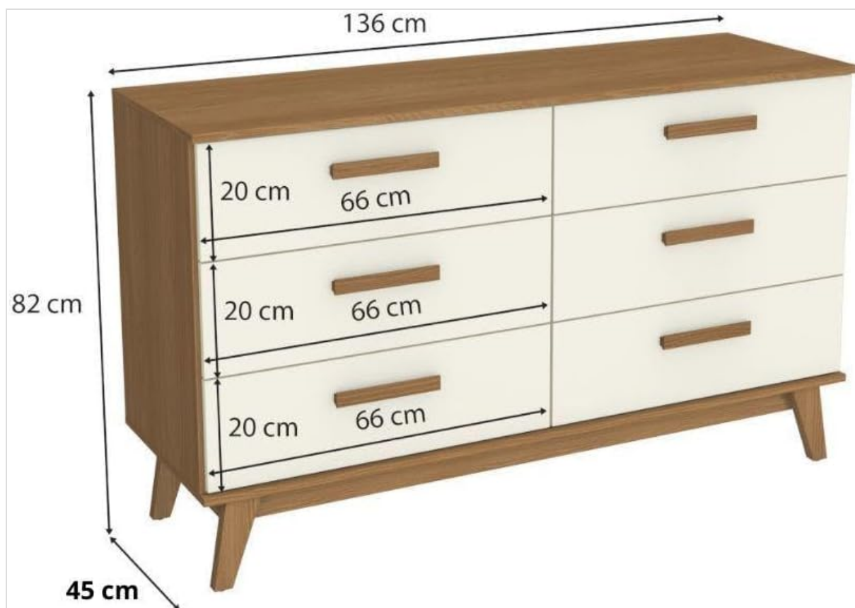
Figure 4.1: Product dimensions for the Kappesberg T268 Chest of Drawers.
