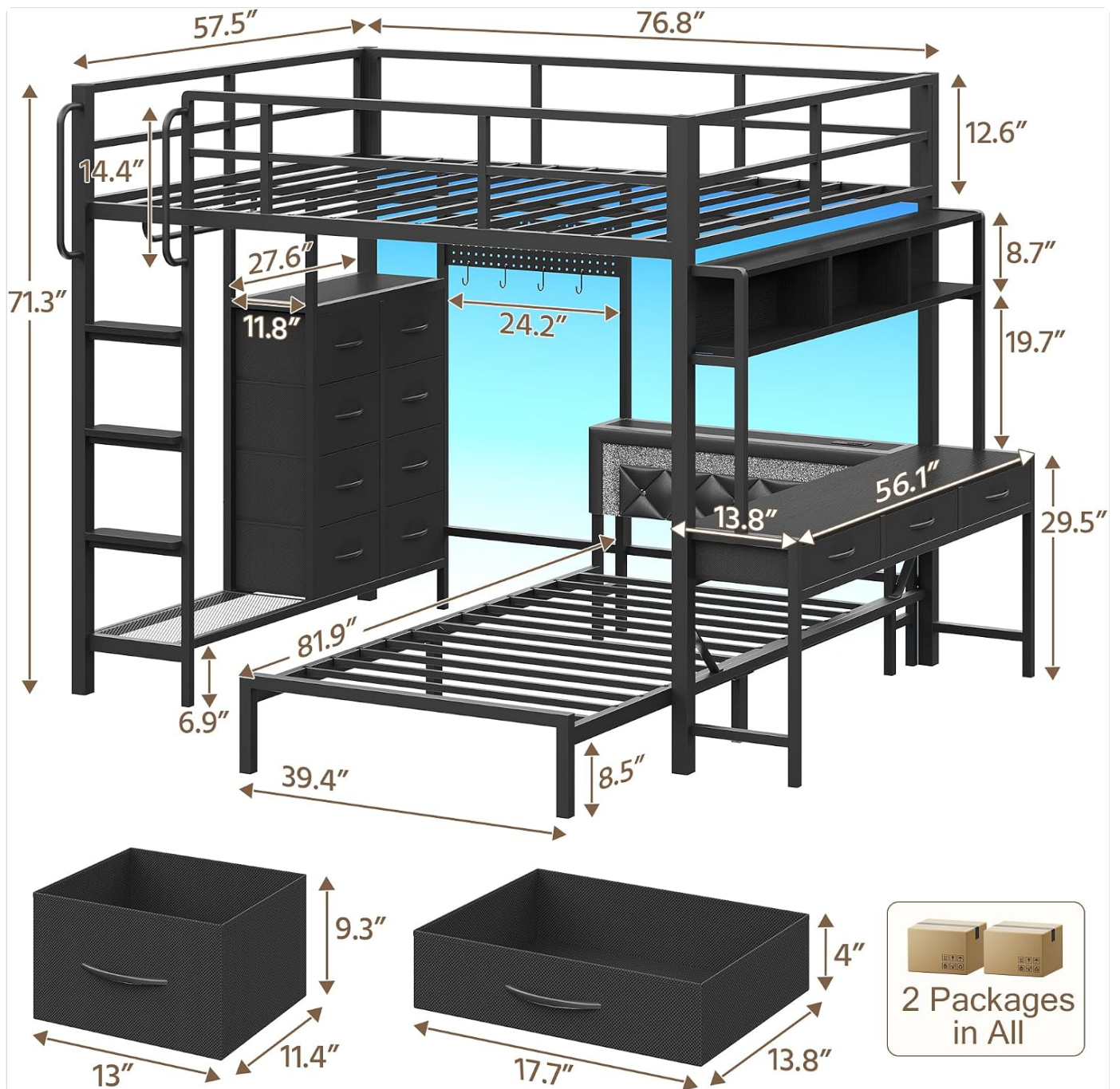
Figure 1: Overall dimensions and key features of the bunk bed.
