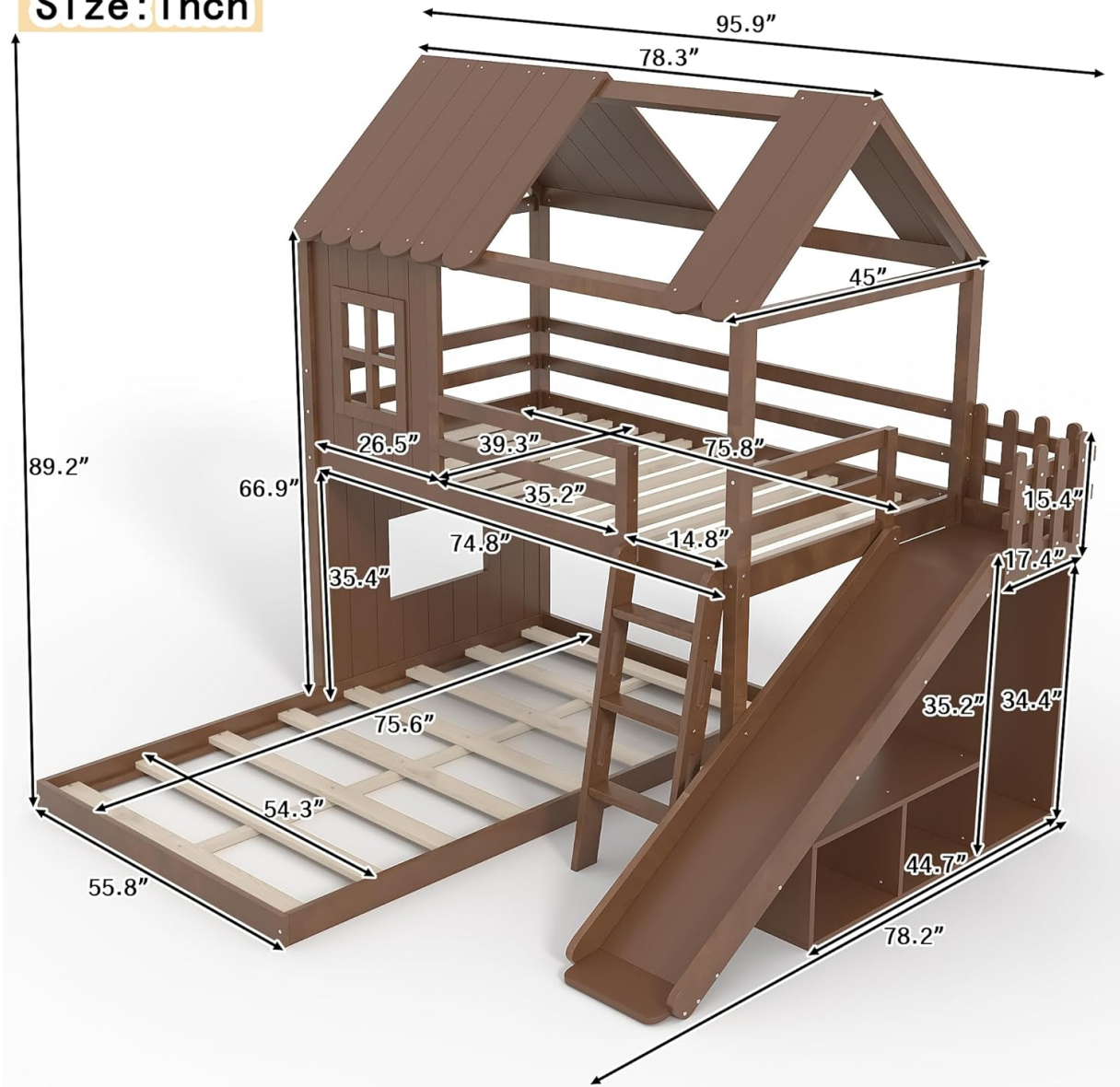
Image 3.1: Detailed dimensions of the bunk bed.
