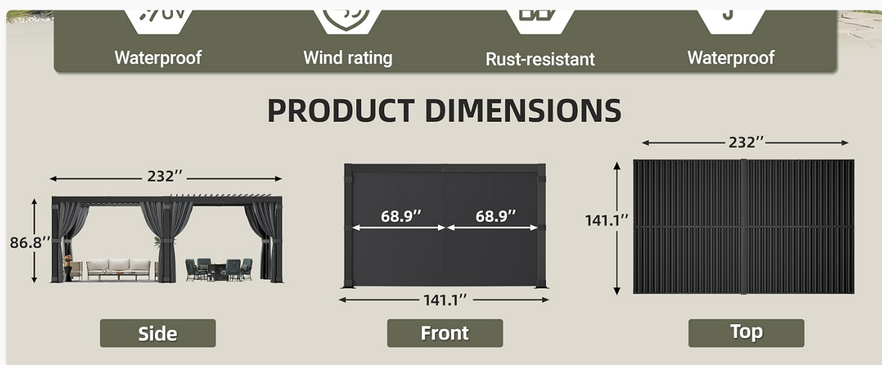
Figure 2: Product dimensions overview.
