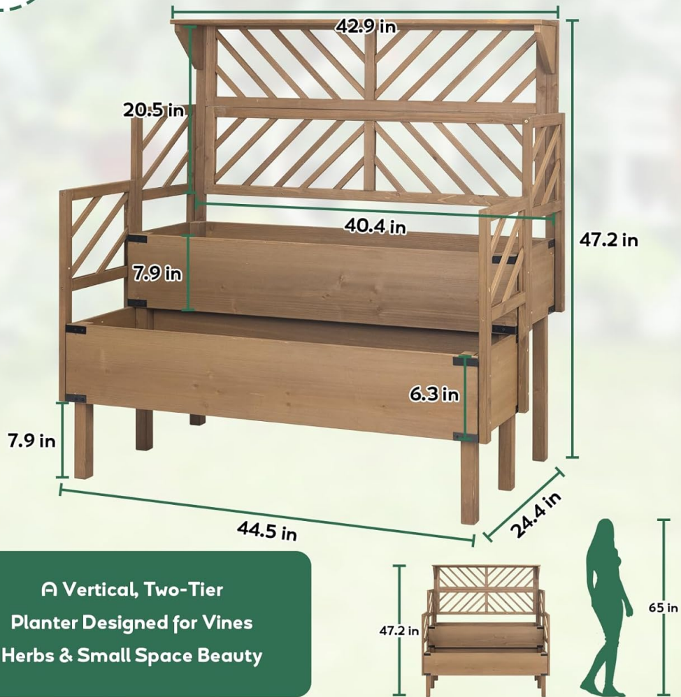
Image: A diagram illustrating the key dimensions of the raised garden bed, including overall height, width, and depth, as well as individual tier measurements.
