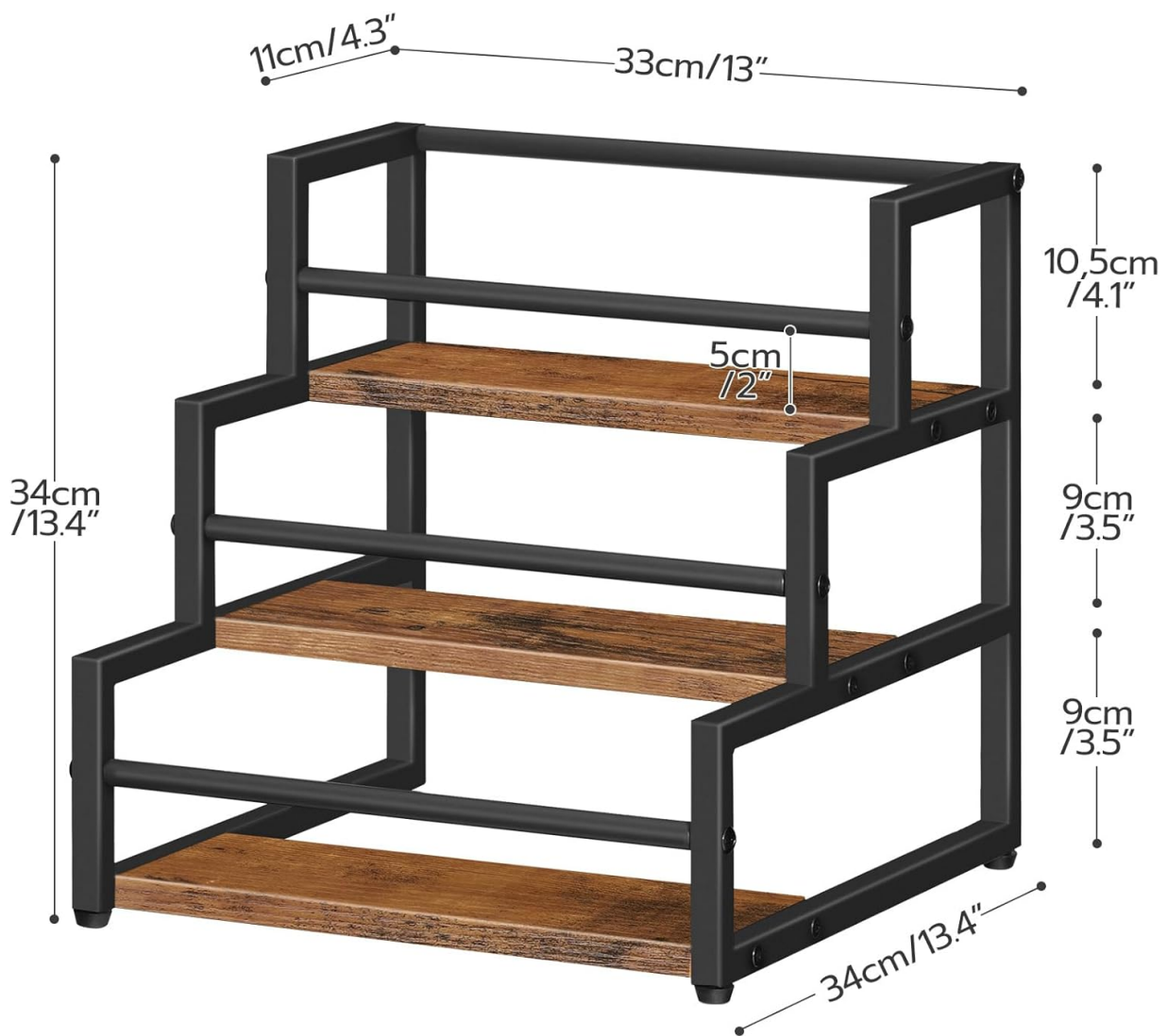
Figure 3.2: Detailed dimensions for the HOOBRO Coffee Syrup Rack (BF38JJ01), illustrating overall length, width, height, and individual shelf heights.
