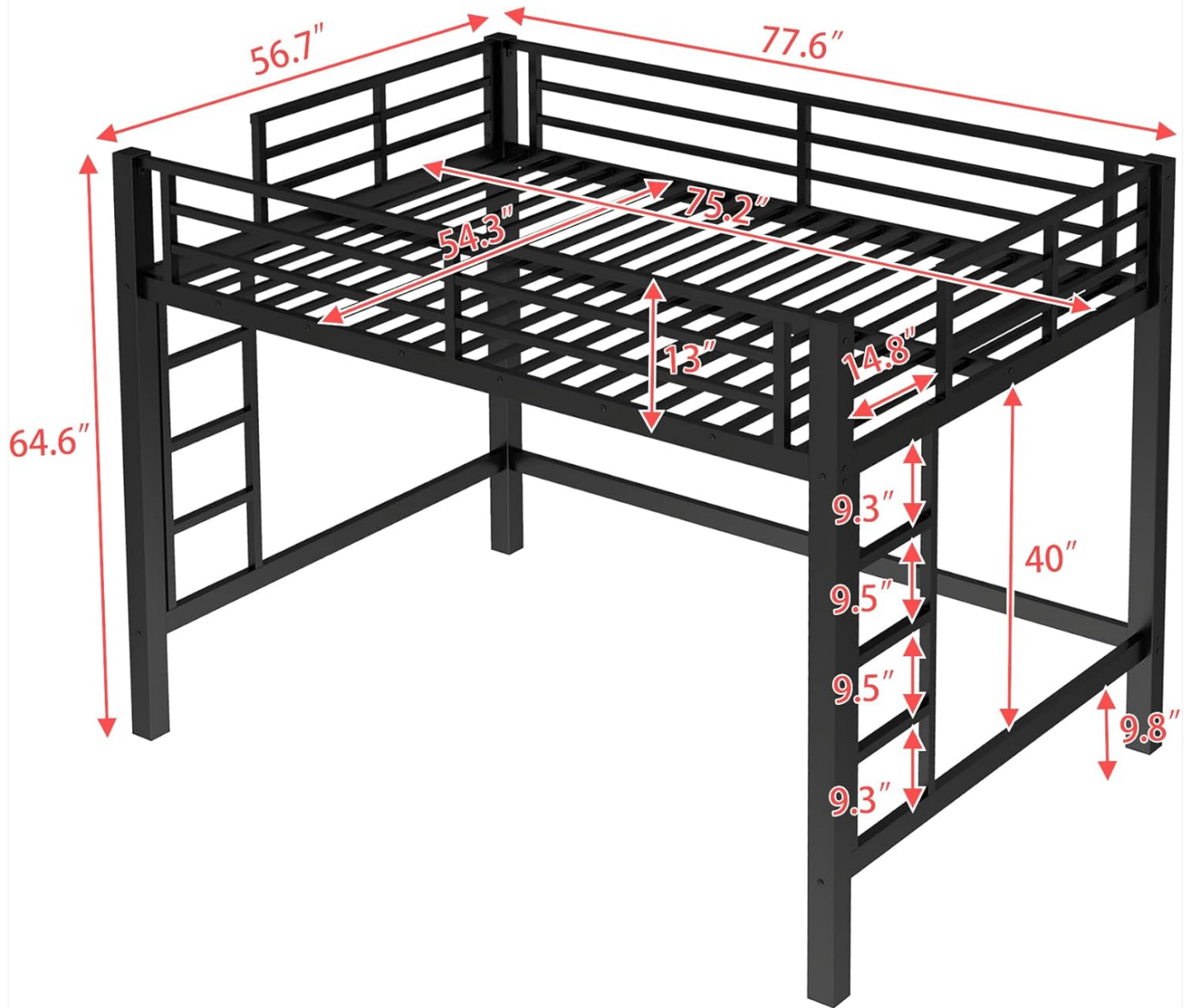
Figure 6: Detailed dimensions of the Bellemave Full Loft Bed in inches.
