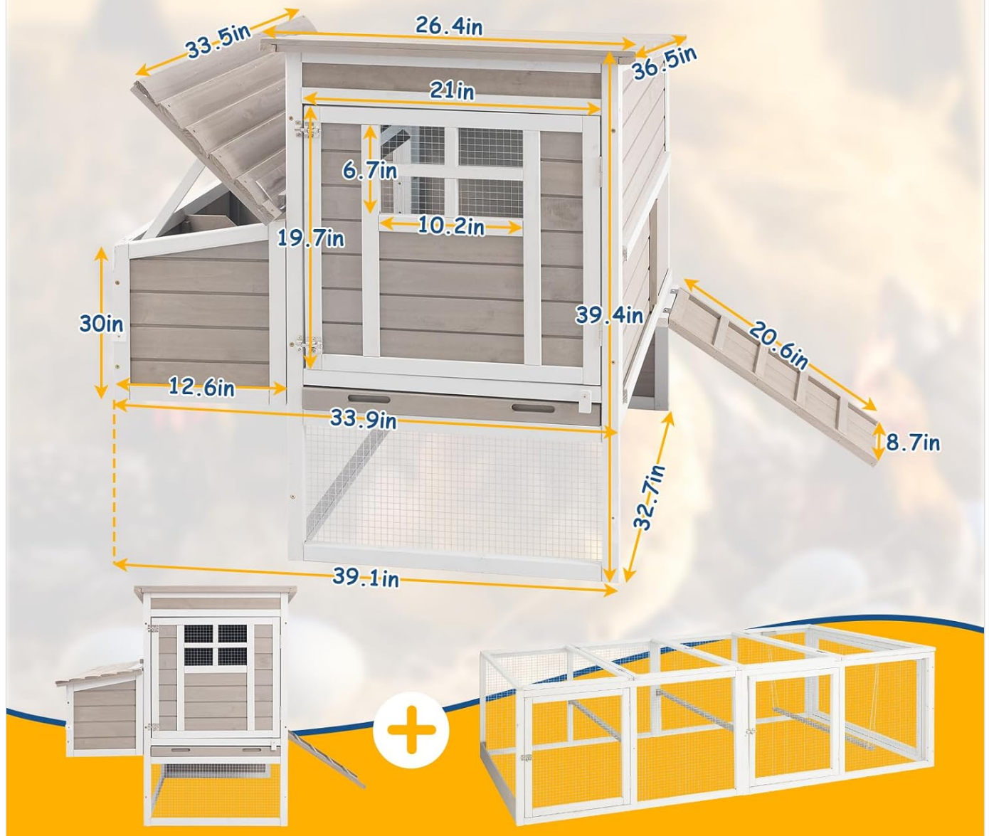
Image: Diagram showing the dimensions of the coop and how it can connect to an expandable run for increased space.
