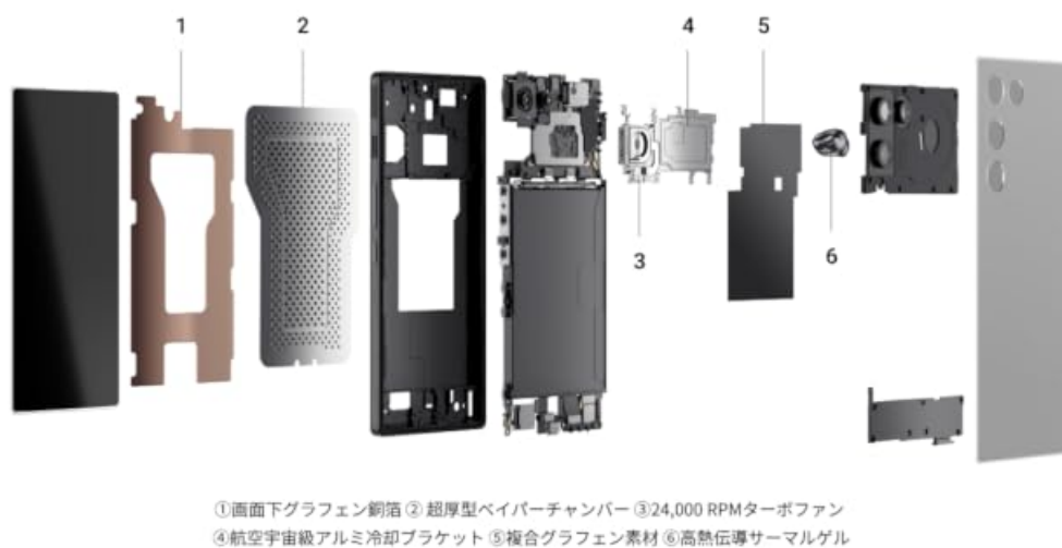
Figure 2.3: Integrated cooling fan and Vapor Chamber for efficient heat dissipation.
